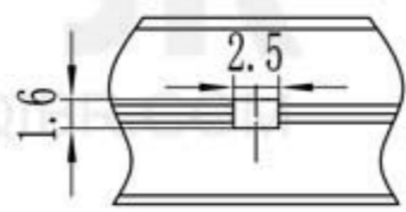
OIL HOLE DETAILS
