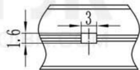
OIL HOLE DETAILS
